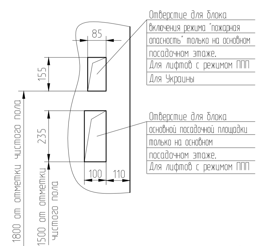
Л-Л (1:10) (2, 4)
