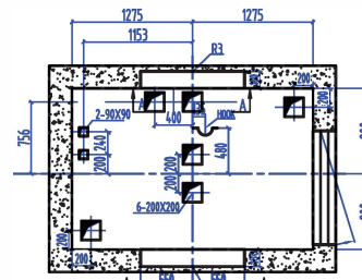
CUTOUTS OF MACHINEROOM
