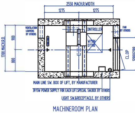
MACHINEROOM PLAN
