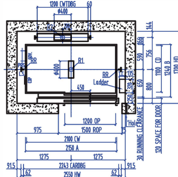
HOISTWAY PLAN
